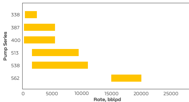
Figure 2. High-rate pumps
